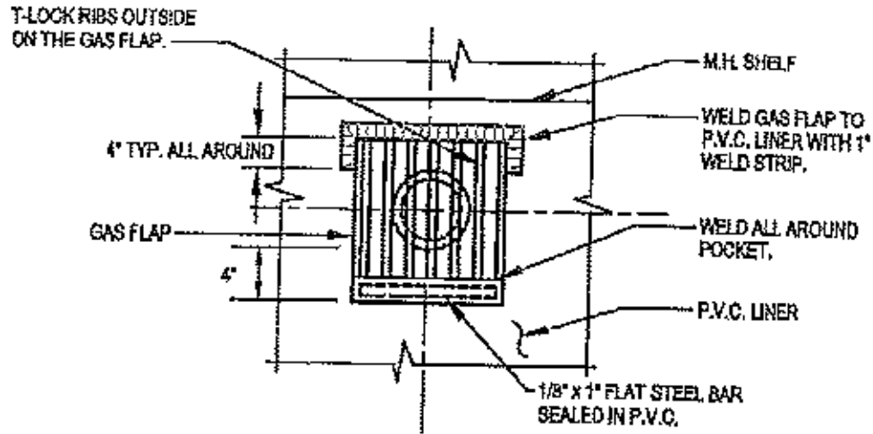
VIEW C-C NOT TO SCALE
