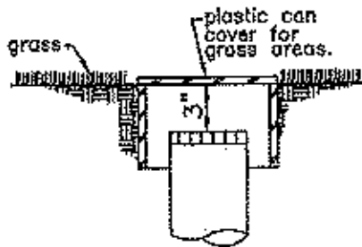
DETAIL-UNPAVED AREA
